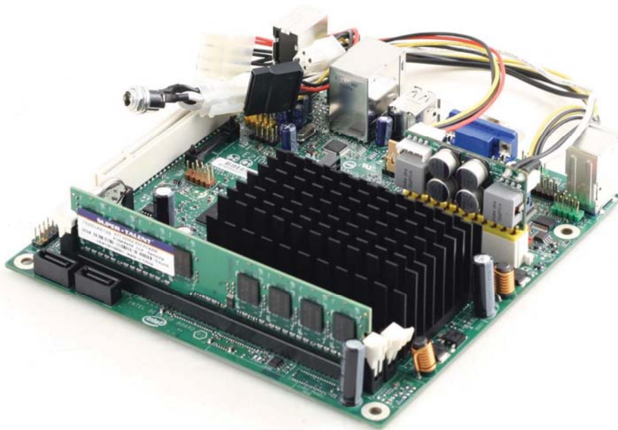
PicoPSU-160-XT shown with the D510MO Intel Motherboard.
